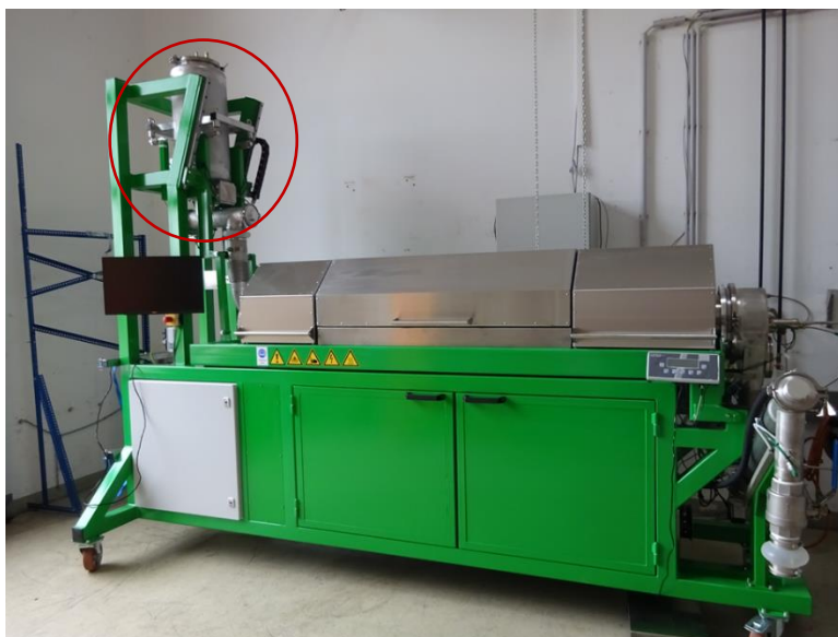
Figure 2: The used rotary kiln system, with the feedstock storage marked in red
