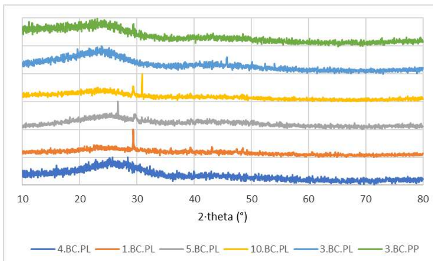
Figure 22: xrd 4. Relative comparison of XRD stacked spectra of the biochar pyrolysis samples made from coffee husks - 1.BC.PL; walnut shells - 3.BC.PL; bran 4.BC.PL; Compost screenings - 5.BC.PL; wood chips from broadleaf forestry sites - 10.BC.PL; walnut shells - 3.BC.PP WS;
