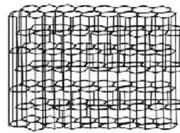
Graphite structure
